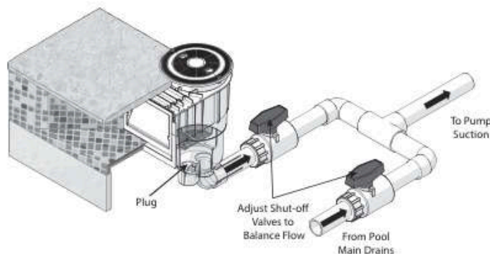
Figure 2: Typical residential installation
