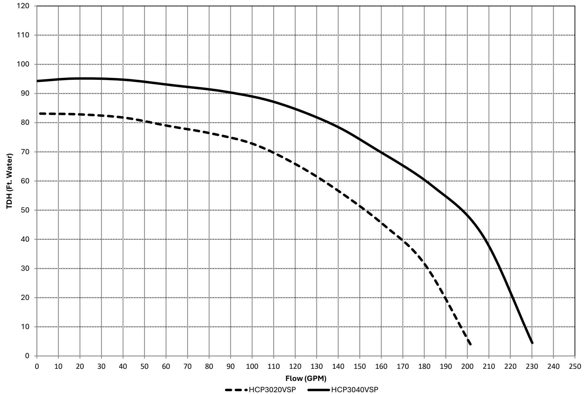
TriStar XL VS Performance Curves
