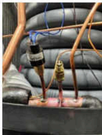
THE L.P. SWITCH HAS BLUE WIRE LEADS
