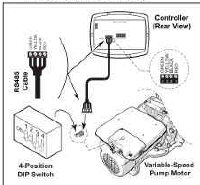
Figure 4. Wiring the Controller to the Variable Speed Pump
