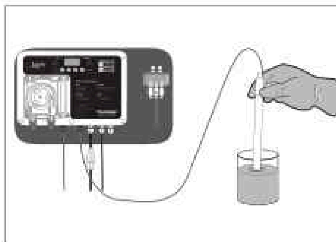
Figure 16. Check Sensors
