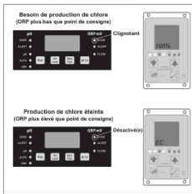
Figure 14. Interfaces TruDose/APUREM
