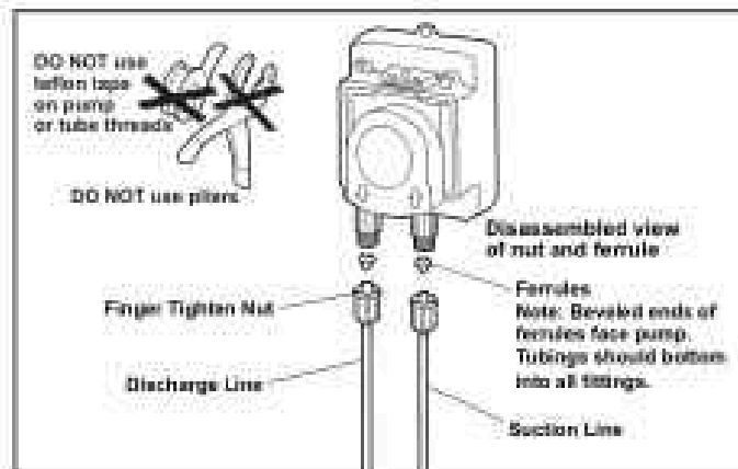
Figure 11. Install Suction Line to Pump Head
