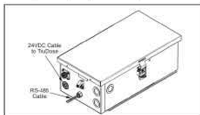
Figure 7. TruClear XL Communication/Power Connection
