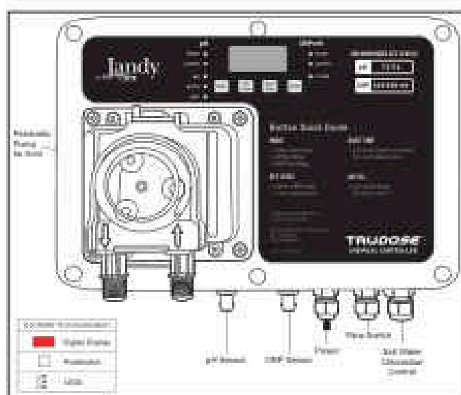
Figure 3. Controller Connections
