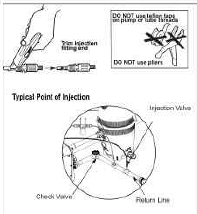
Figure 13. Install Discharge Line to Pump Head and Injection Point
