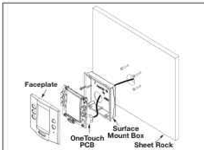
Figure 24. OneTouch™ Surface Mount Installation
