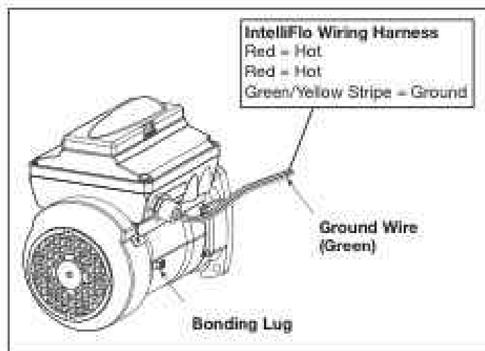
Figure 11. Pentair External Bonding
