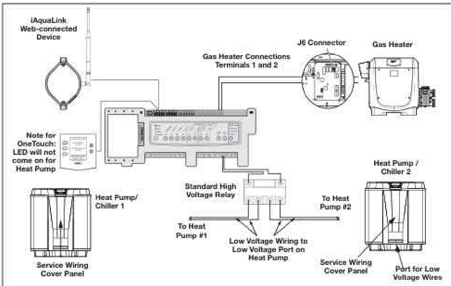
Figure 19. Heater and Heat Pump/Chiller Wiring
