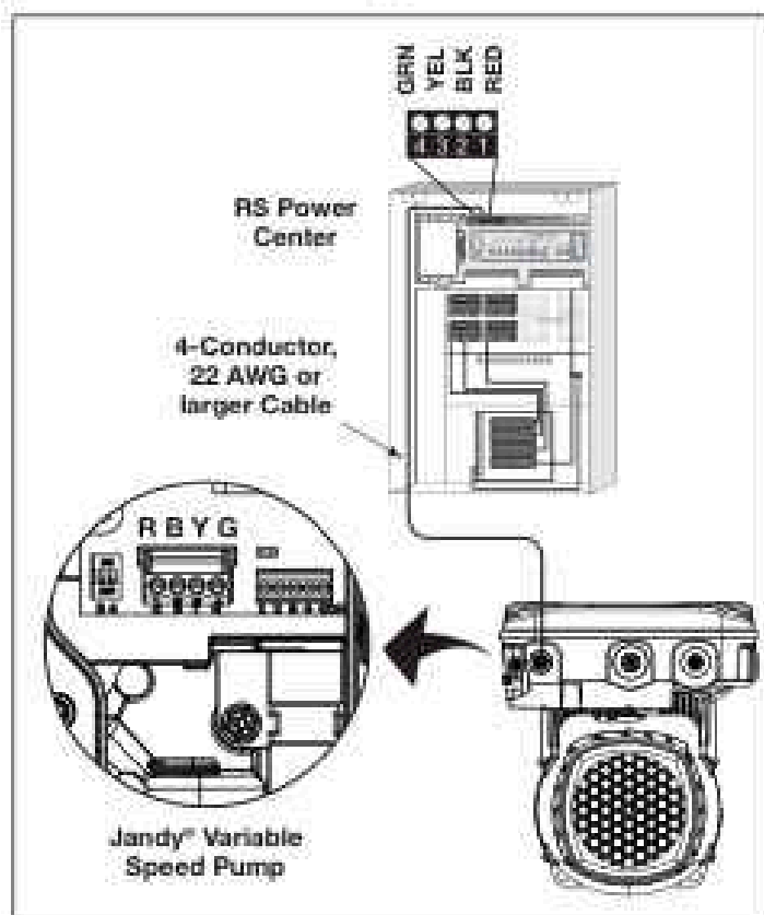
Figure 14. Low Voltage Wiring for Jandy Variable Speed Pump
