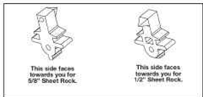
Figure 27. Cleat Orientation
