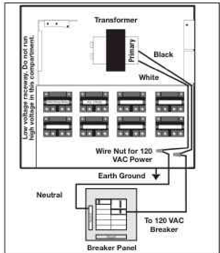
Figure 3. Standard Power Center
