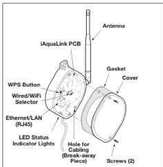
Figure 32. iAquaLink Device PCB Components
