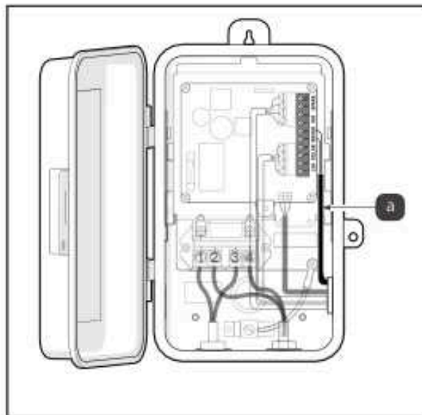
Figure 7. Connect Low Voltage Wires
