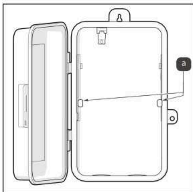
Figure 10. Intermatic® Retaining Ears Location
