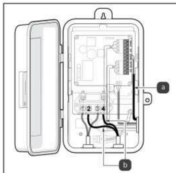
Figure 13. Connect Load Input Cables
