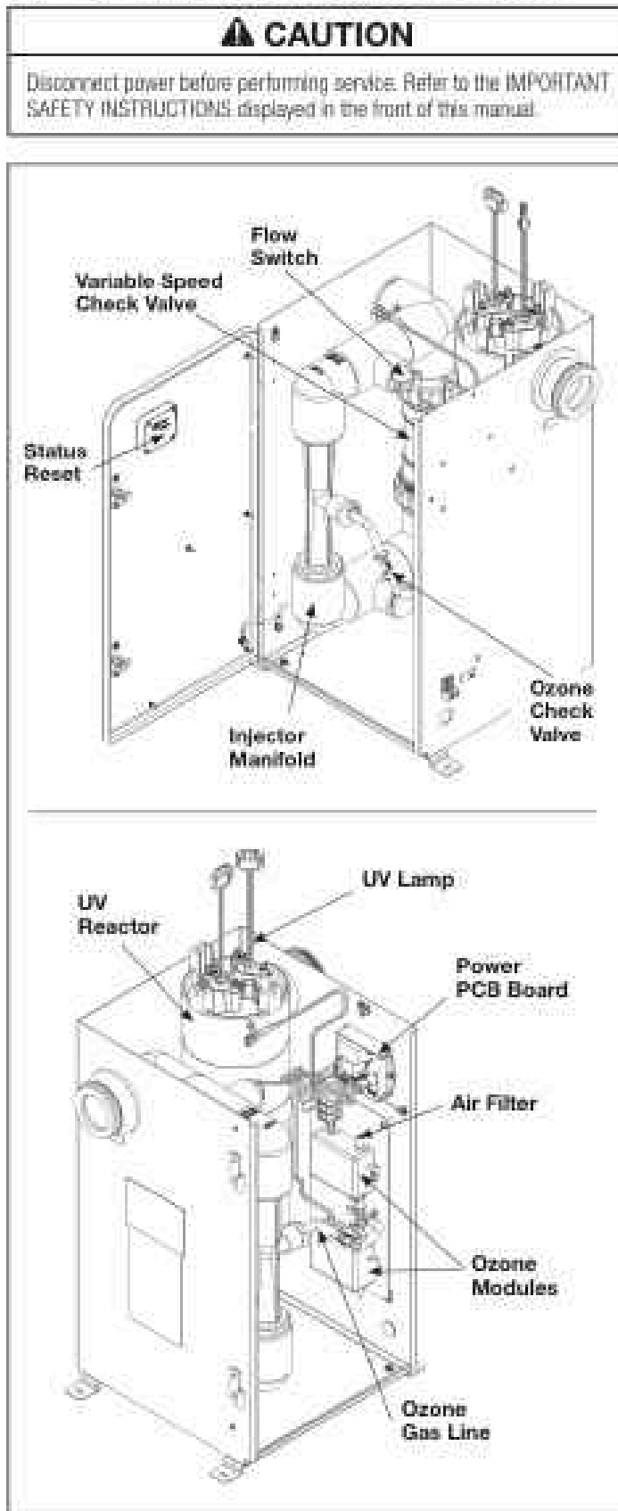
Figure 10. Jandy AOP Electro-Mechanical Overview (JAOPX350 Shown)
