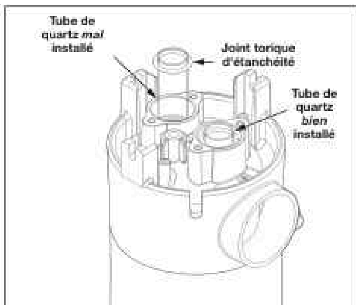
Figure 16. Installation du tube de quartz UV
