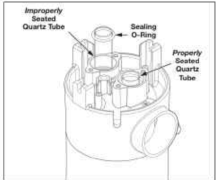
Figure 16. UV Quartz Tube Installation
