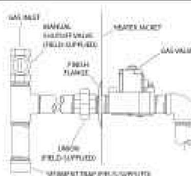
Figure 10. Gas Line Sediment Trap
