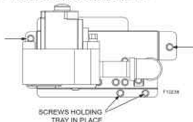
Figure 42. Gas Valve Removal
