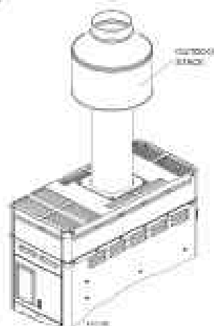
Figure 7. Outdoor Stack
