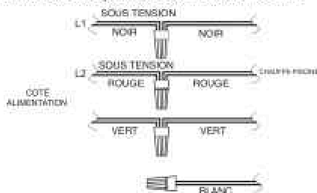
Figure 18. Raccordements à 240 VCA
