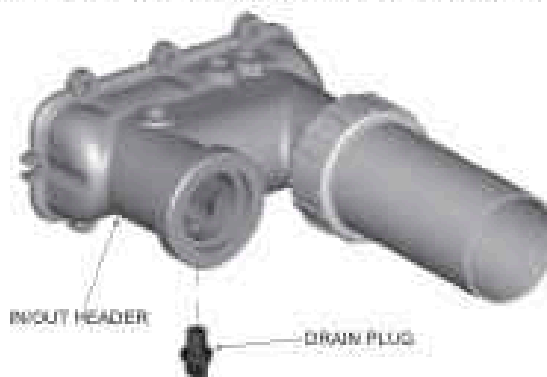
Figure 35. In/Out Header Drain Plug Location
