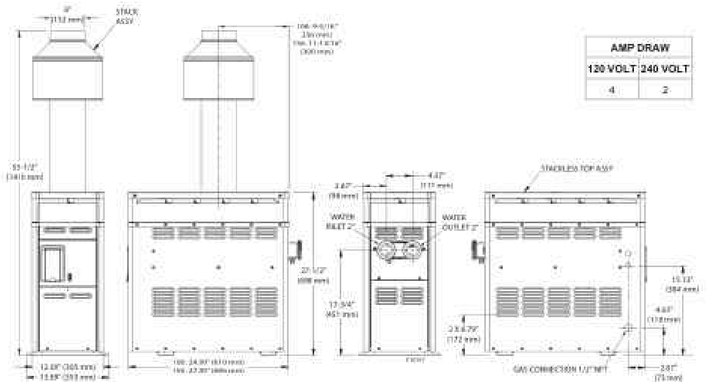
Figure 4. Heater Dimensions
