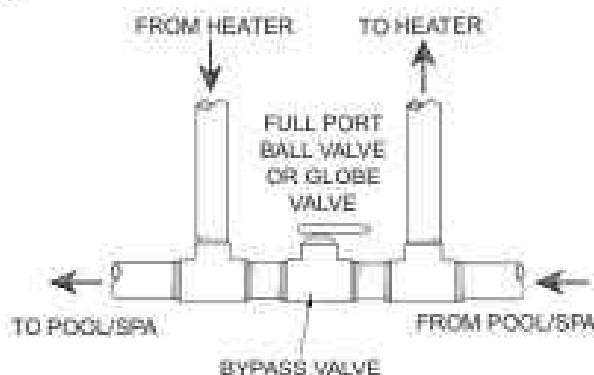
Figure 16. Auxiliary Bypass Valve
