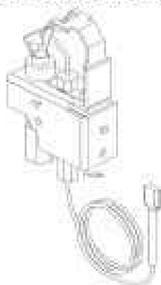
Figure 43. Spark-to-Hood Pilot
