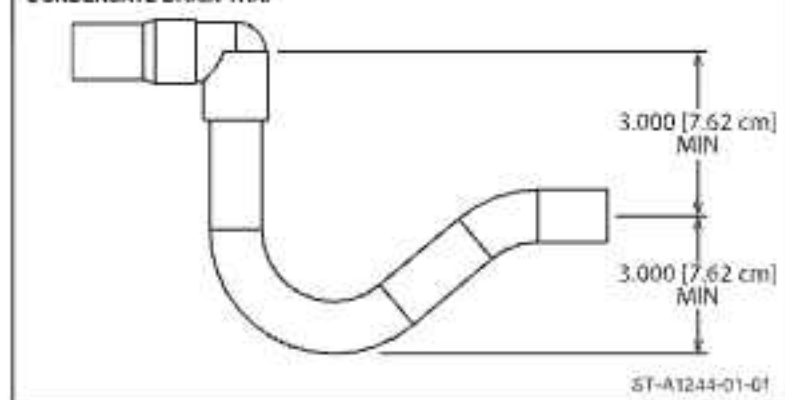
FIGURE 13 CONDENSATE DRAIN TRAP
