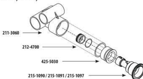
Tee Body Assembly
