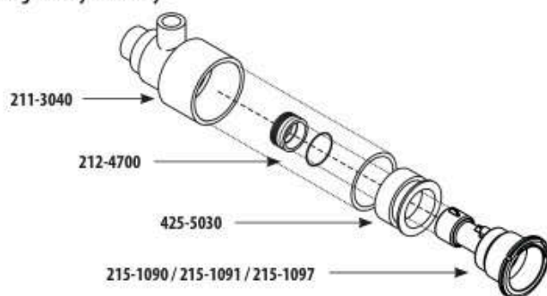
Straight Body Assembly
