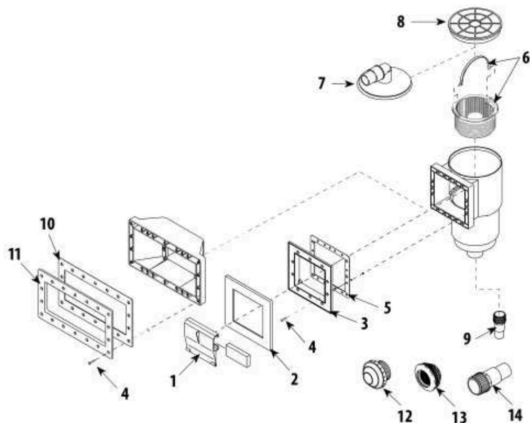
Flo-Pro II Above-Ground Skimmer Replacement Parts
