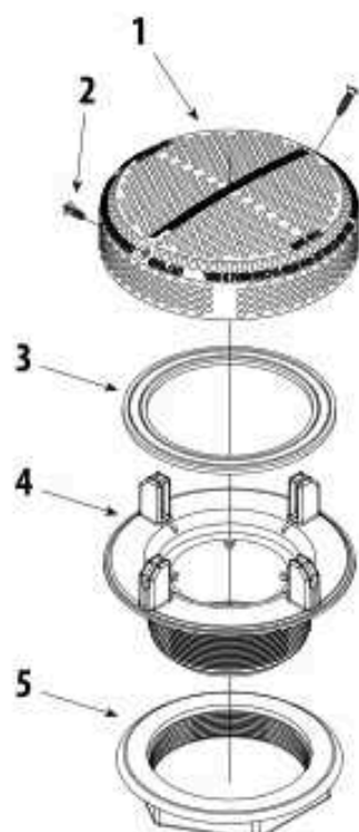
Super Hi-Flo Suction
