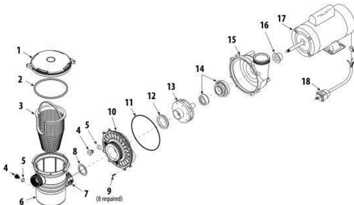
Hi-Flo Side Discharge Pump Replacement Parts
