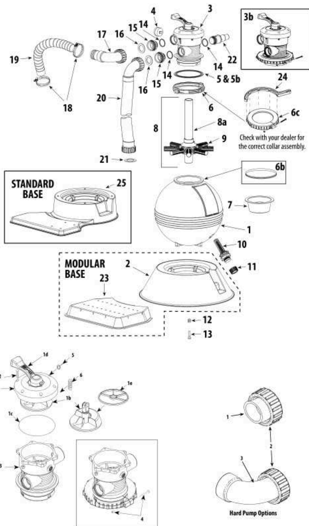
Multi-Port Valve Assembly
