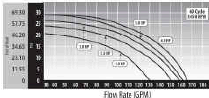
CSA Hi-Flo II Side Discharge 48-Frame Above Ground Pool Pumps
