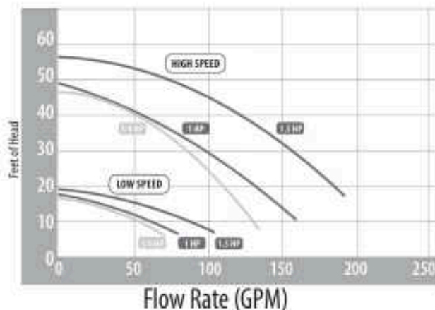
Hi-Flo II Side Discharge 48-Frame Above Ground Pool Pump and Trap
