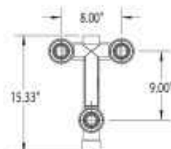
9" Gunite - 3-Jet Manifold
