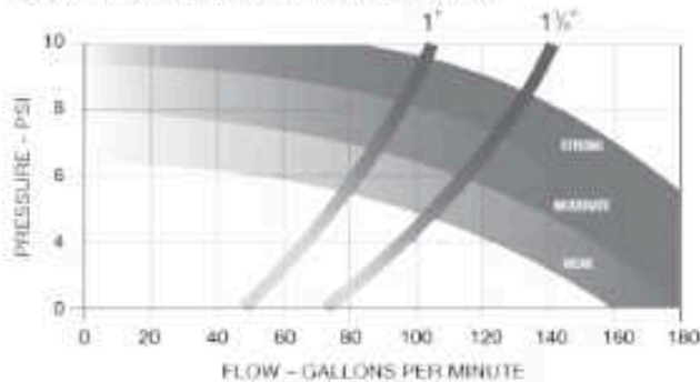
POWER STREAM JET FLOW CURVE
