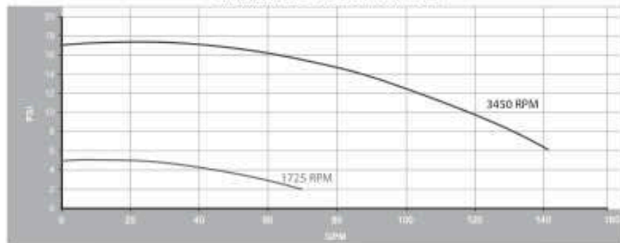
WATERWAY EX2, 9.5/3.2 A, 115V, 1.0 BHP
