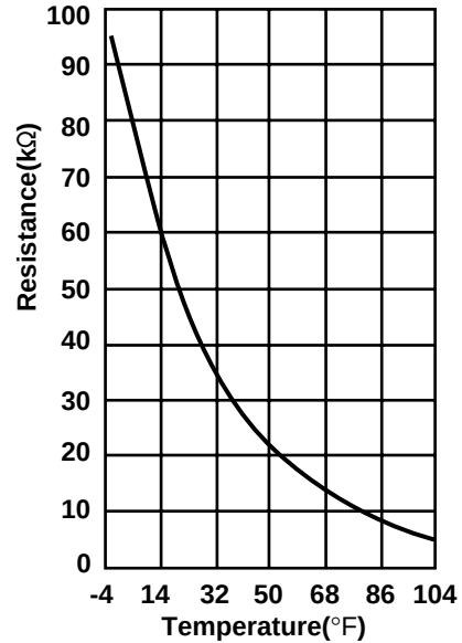
Defrost thermistor (RT61) Ambient temperature thermistor (RT63)
