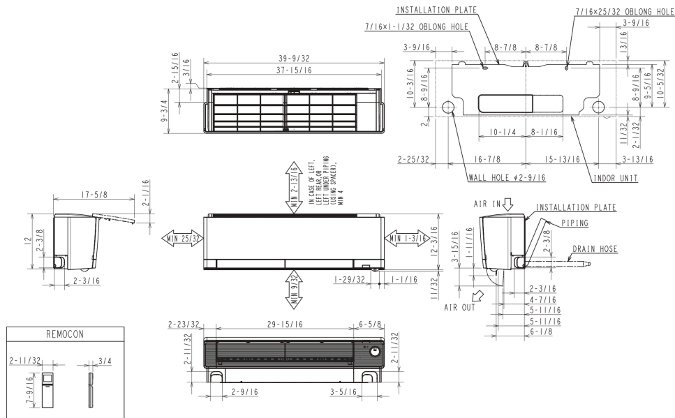
MSZ-FX06/09/12NL
