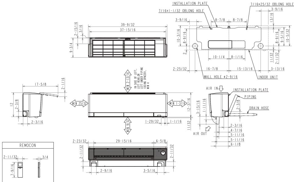
MSZ-FX06/09/12NL
