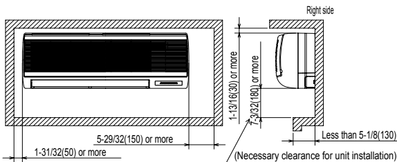
Service space required around indoor unit
