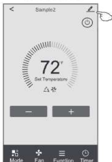
Control form1
